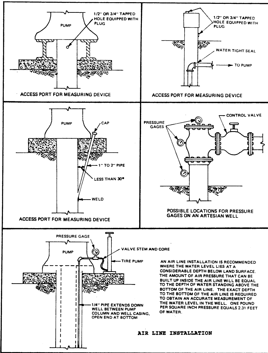
Figure 13: Suggested Methods for Installing Access Ports and Pressure Gages for Measuring Water Levels in Wells
